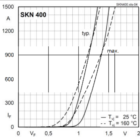
Fig. 5 Forward characteristics
