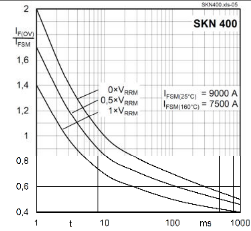
Fig. 6 Surge overload current vs. time
